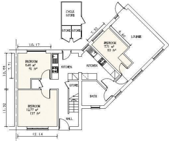
GROUND FLOOR PLANS
